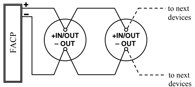
ND-751T-E Wiring Diagram
